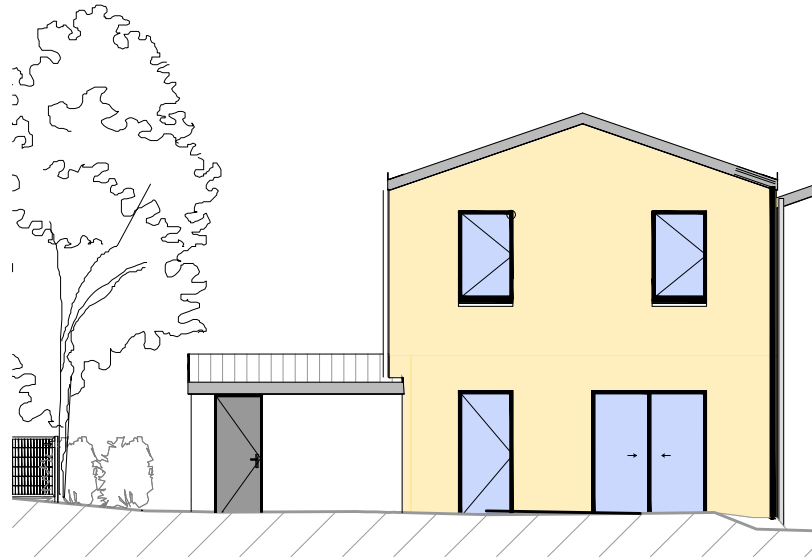
Facade Sud
