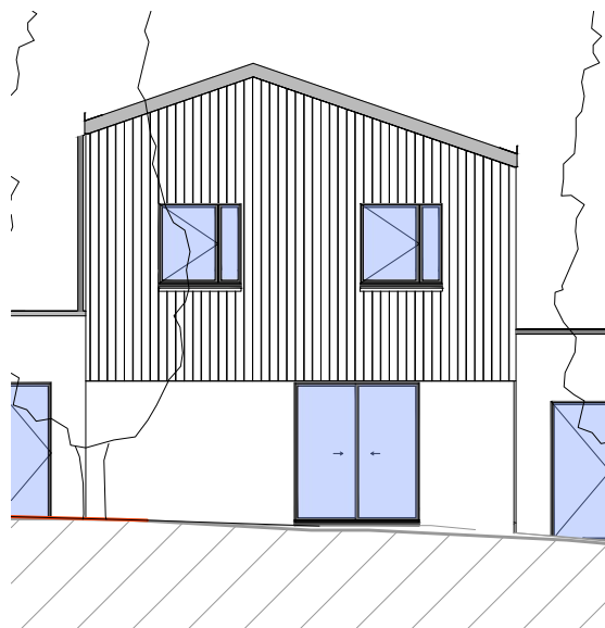
Facade Sud
