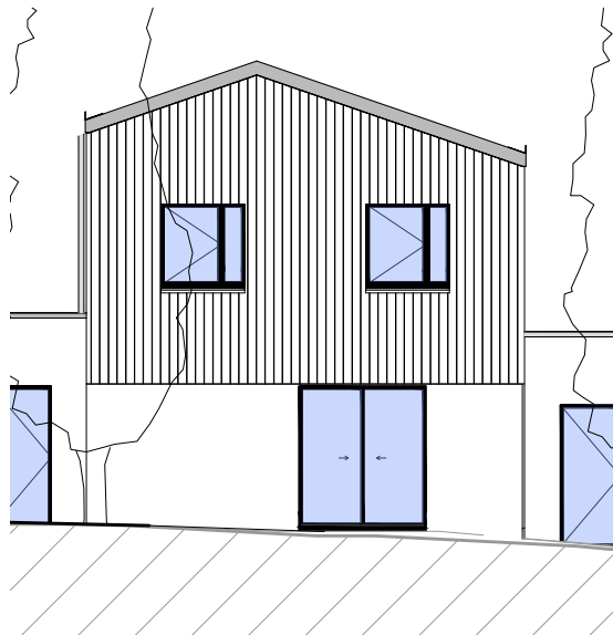
Facade Sud
